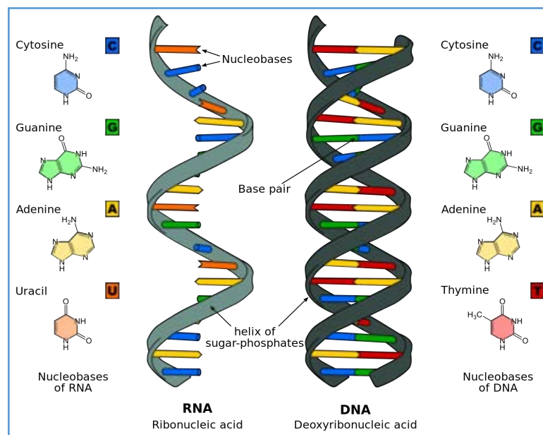
Figure 1.12 A DNA molecule showing the base pairing between adenine (A), thymine (T), cytosine (C) and guanine (G). The DNA contains a triplet code where the base pairs are read in groups of three, each triplet coding for an amino acid. The DNA codes for proteins which are then used to create and maintain an organism.
