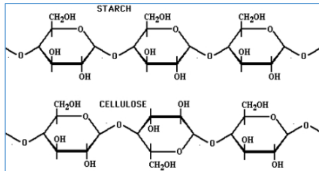
Figure 1.8 Both starch and cellulose are composed of long strands of glucose molecules, the difference being the orientation of the glucose molecules in the chain.
